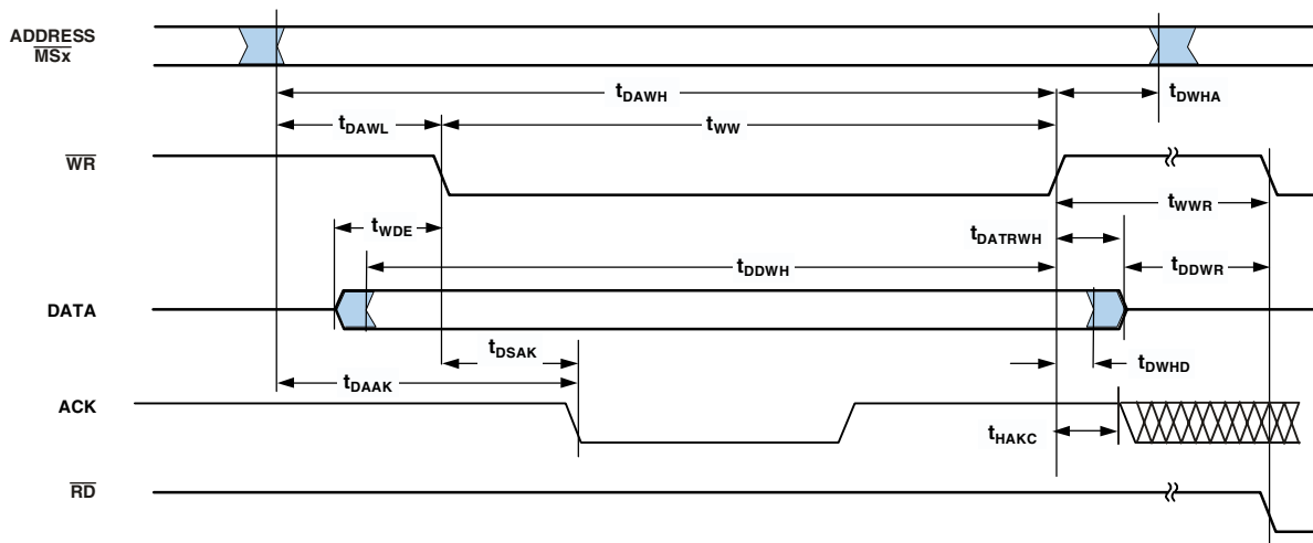
Figure 15. Memory Write – Bus Master
